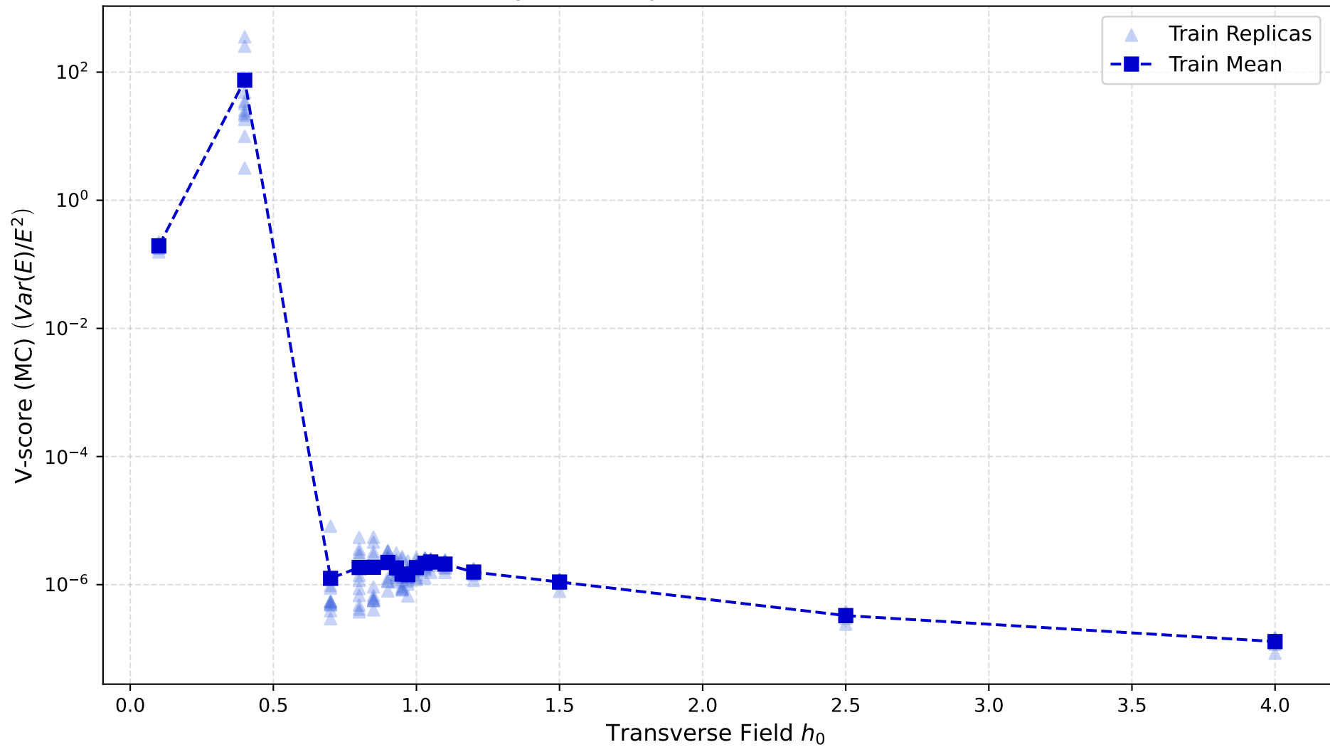
Accuracy Landscape (MC Est.): V-score (L=80)
