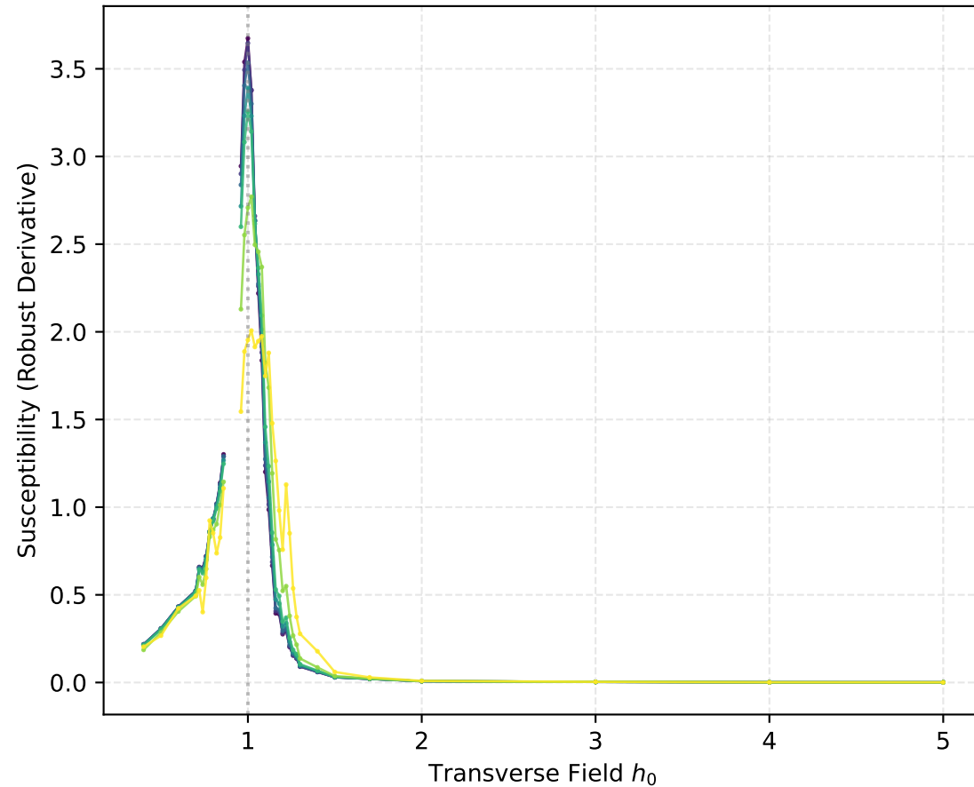
Derivative of Mean M_z^2 (span=1)
