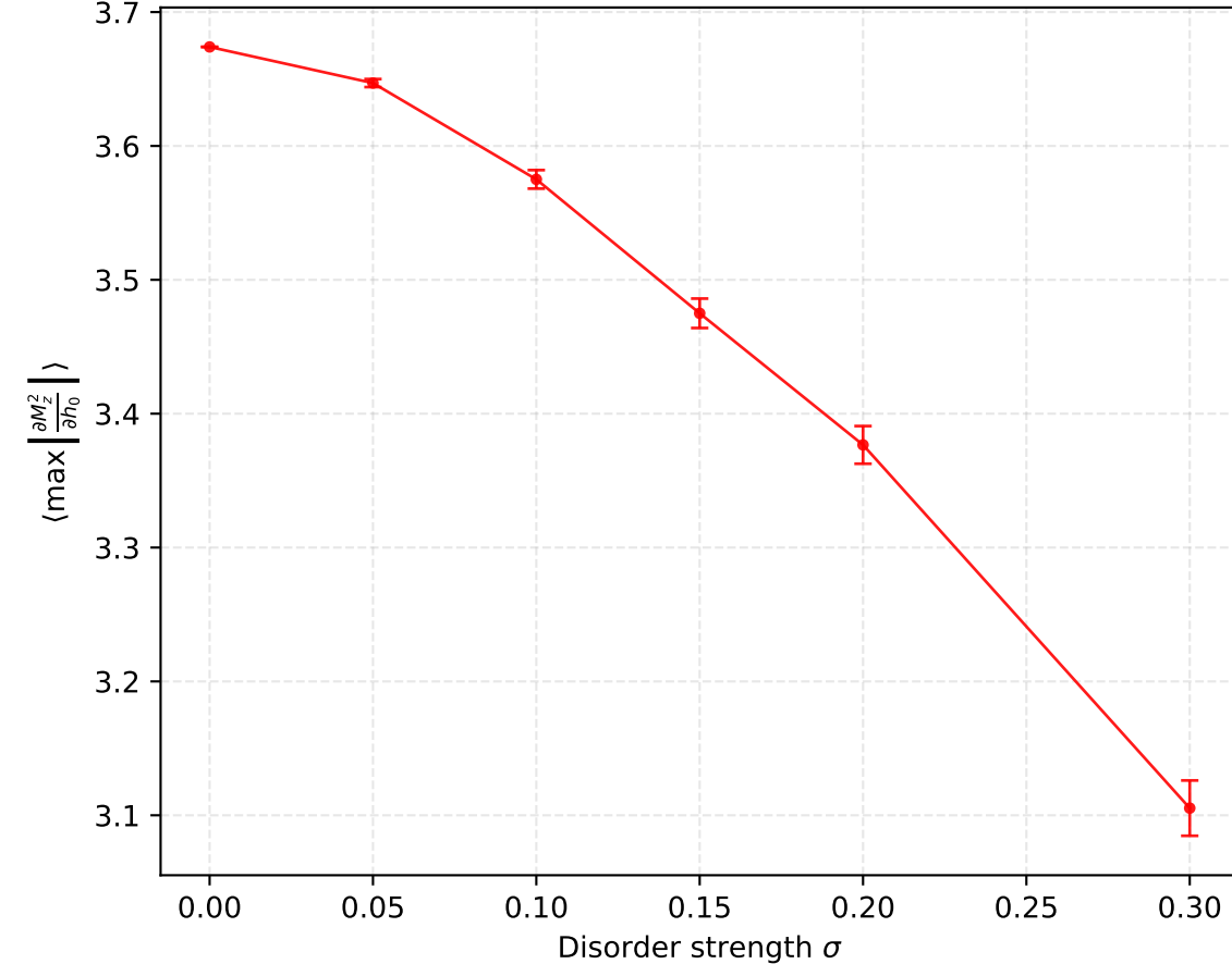
Mean of Max Derivatives ( h_0 \in [0.5, 1.5] )
