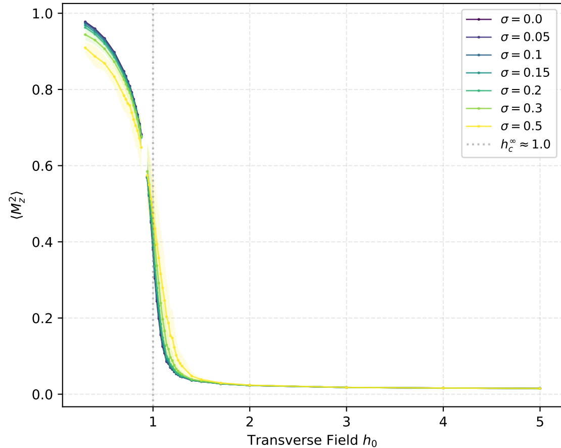
Mean Squared Magnetization — 1D L = 80 (80 spins)
