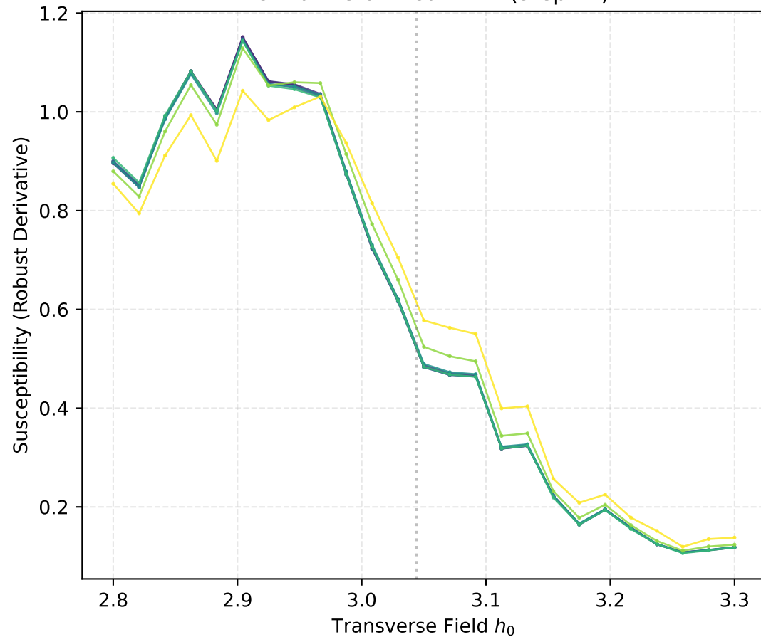
Derivative of Mean M_z^2 (step=2)
