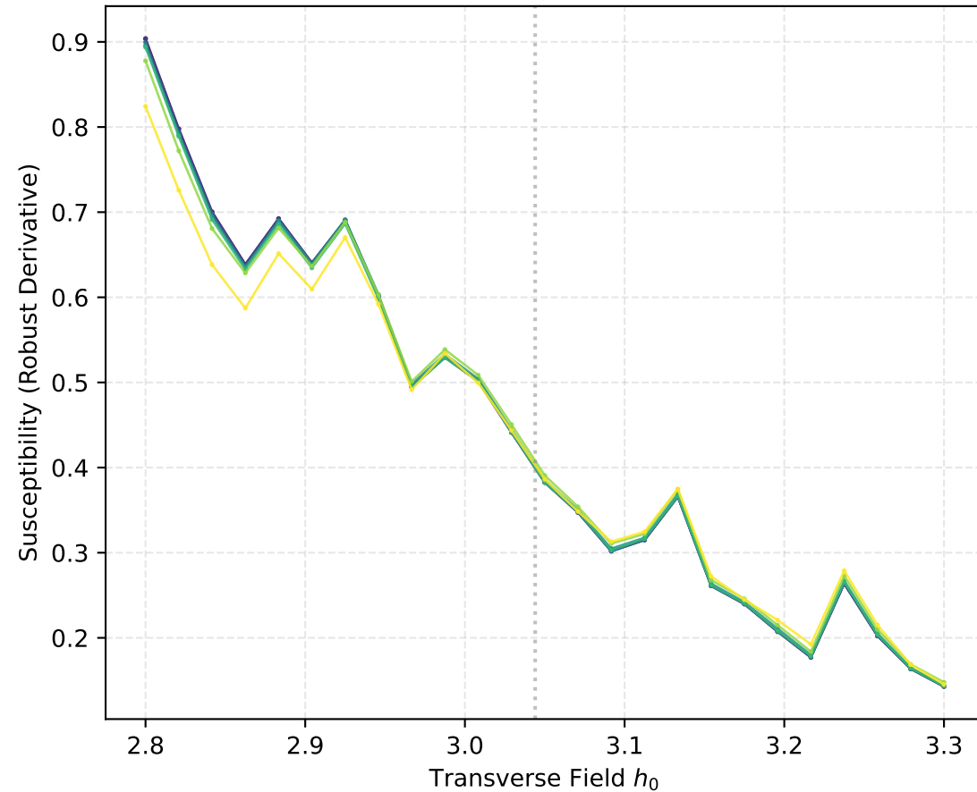
Derivative of Mean M_z^2 (step=2)
