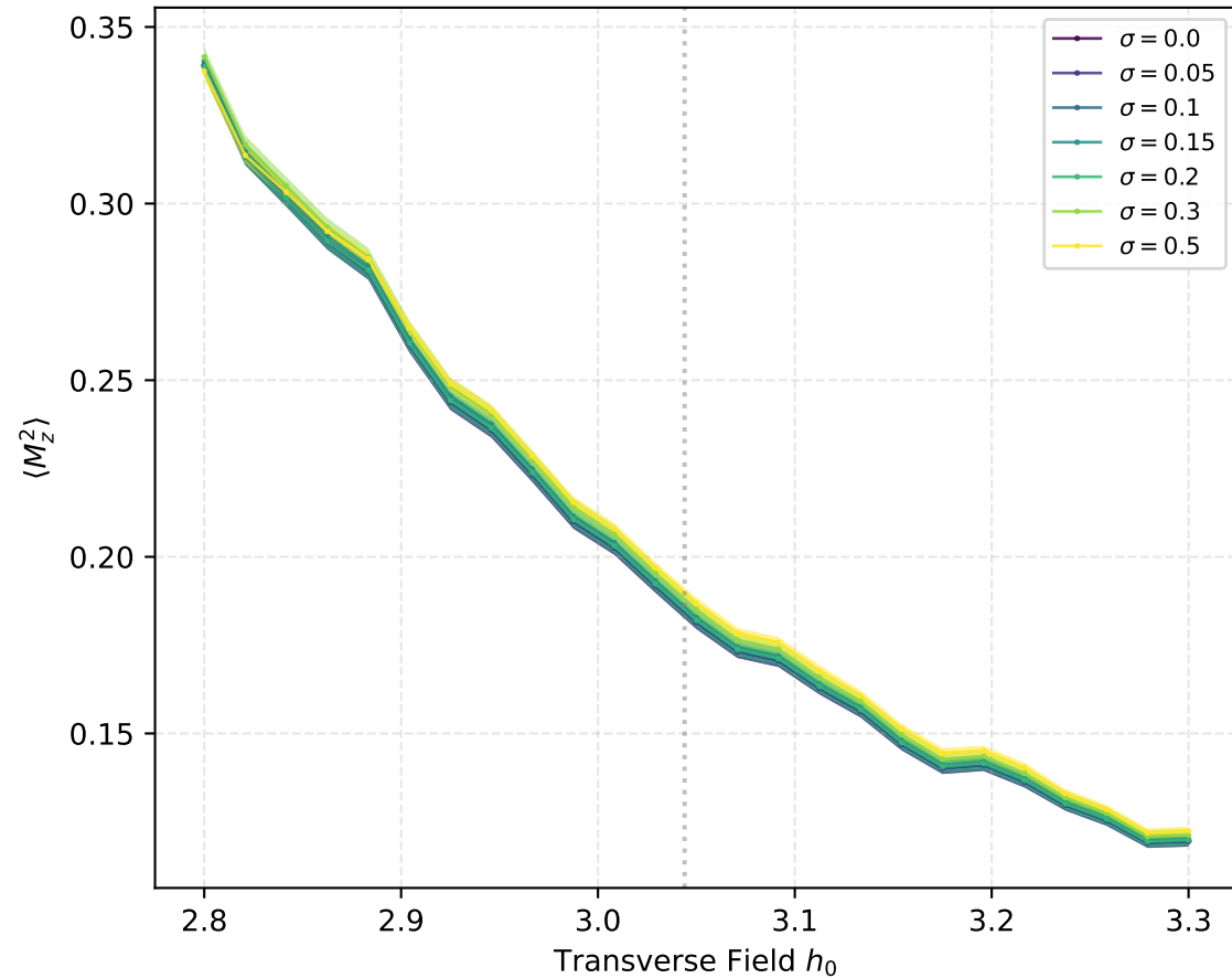
Mean Squared Magnetization — 2D L = 6 (36 spins)
