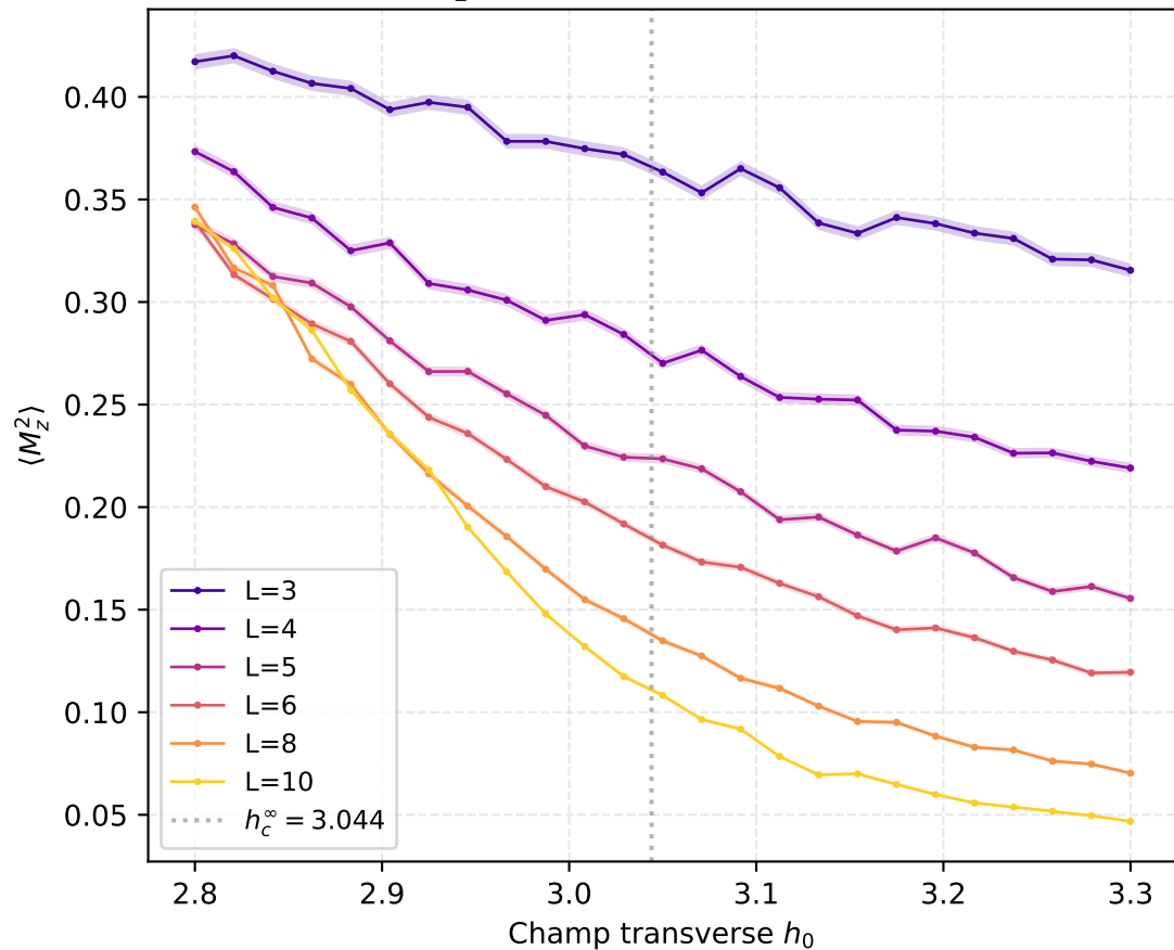
M_Z^2 — \sigma = 0.0 , toutes tailles
