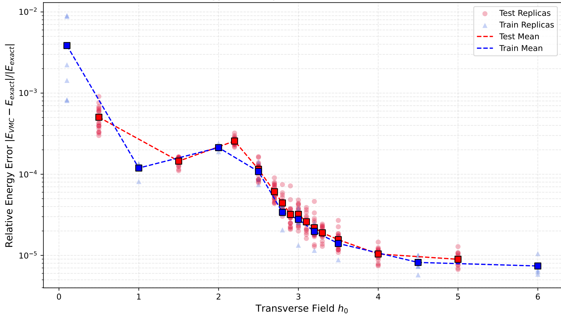
Energy Accuracy: Train vs Test (Grid=4x4)
