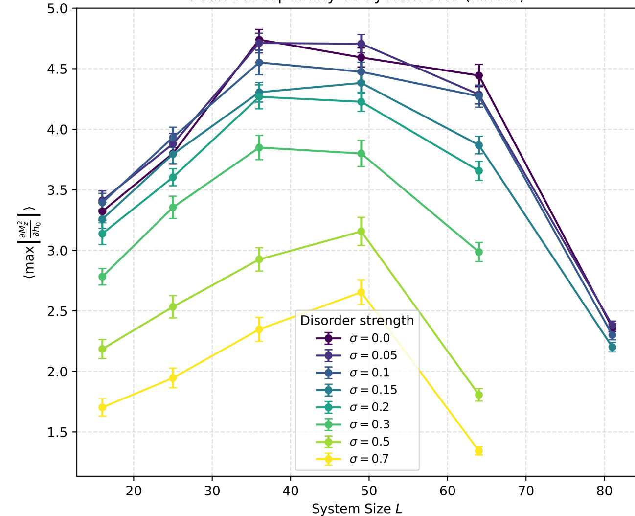
Peak Susceptibility vs System Size (Linear)
