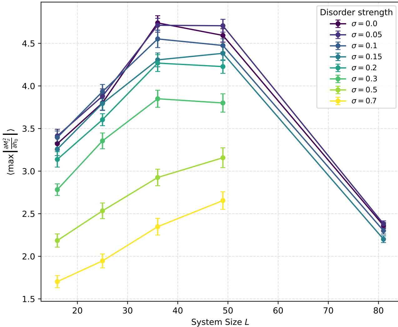
Peak Susceptibility vs System Size (Linear)
