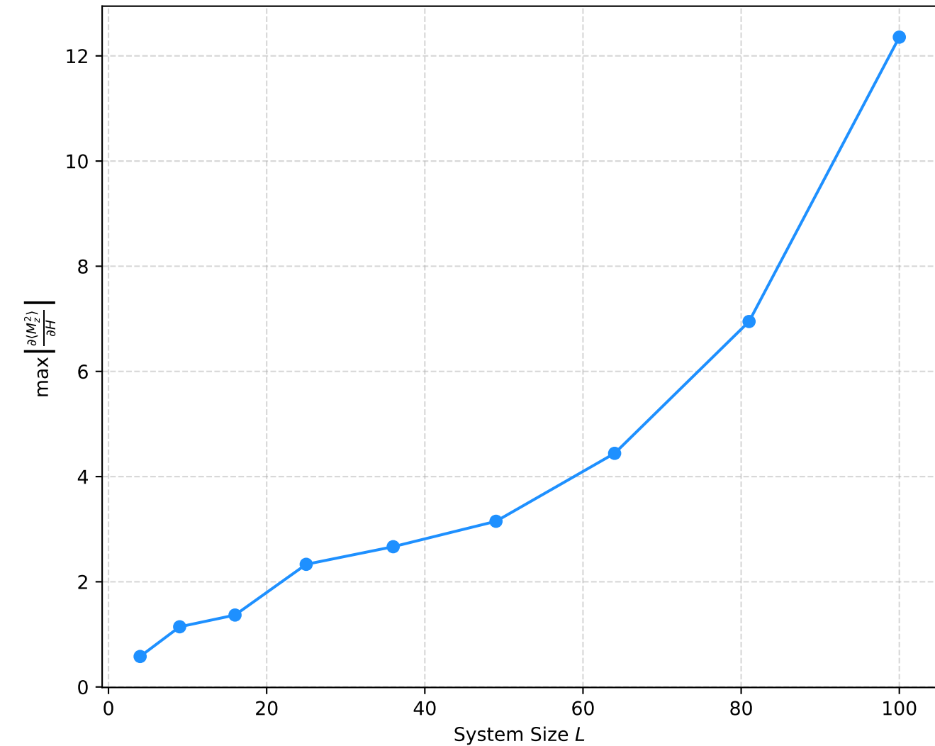
Peak Susceptibility vs System Size (Pure System)
