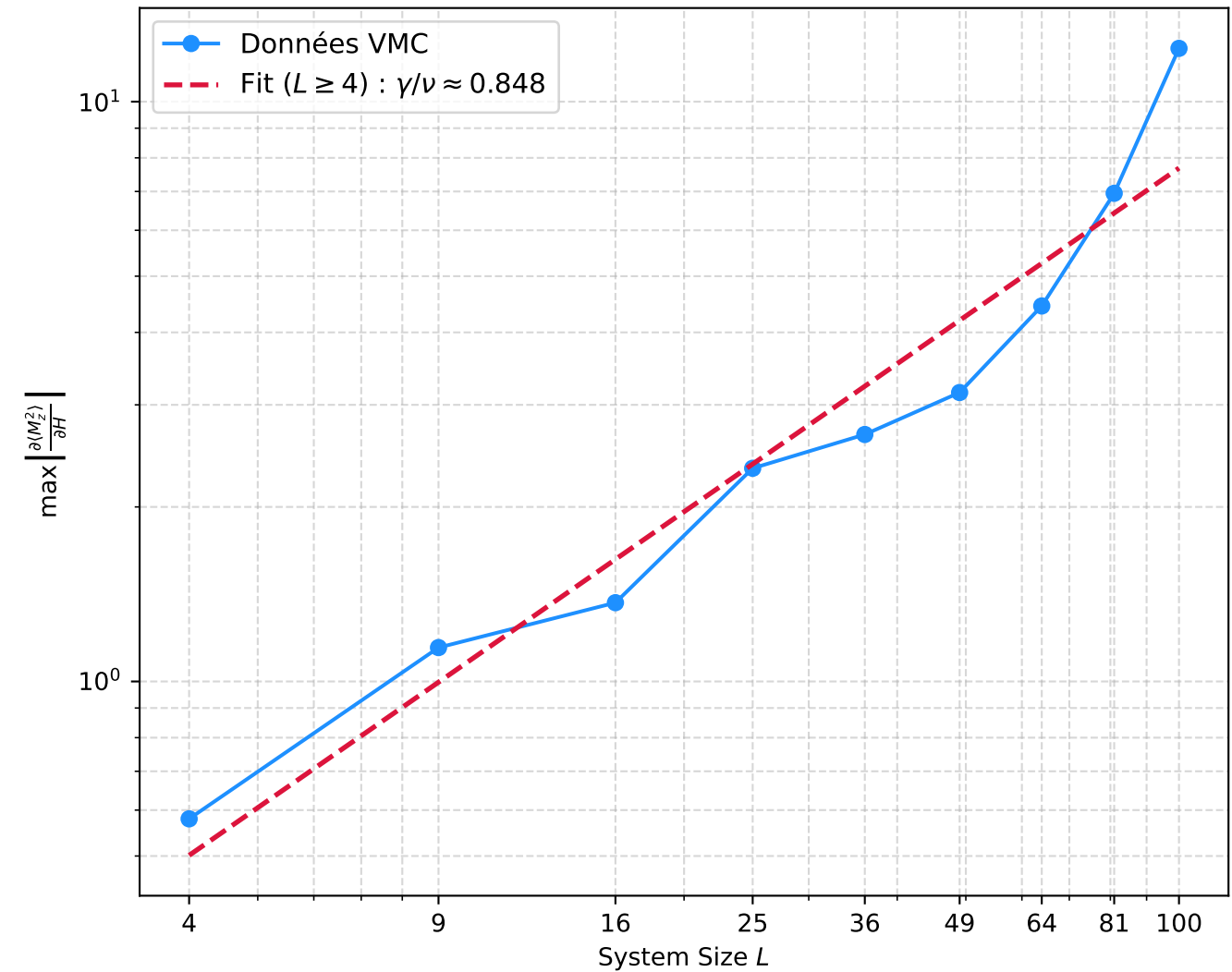
Peak Susceptibility vs System Size (Log-Log)
