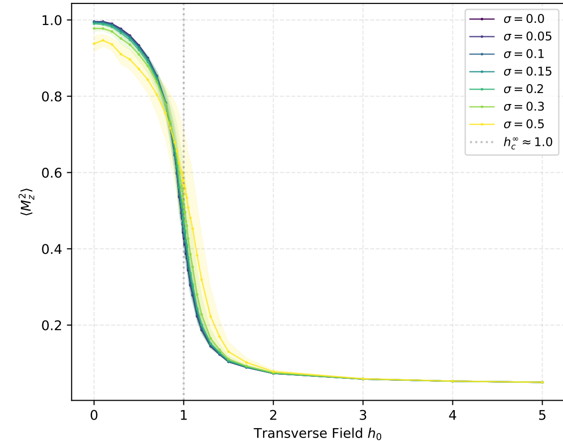
Mean Squared Magnetization — 1D L = 25 (25 spins)
