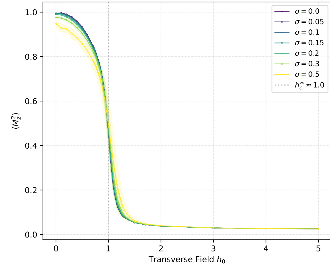
Mean Squared Magnetization — 1D L = 49 (49 spins)
