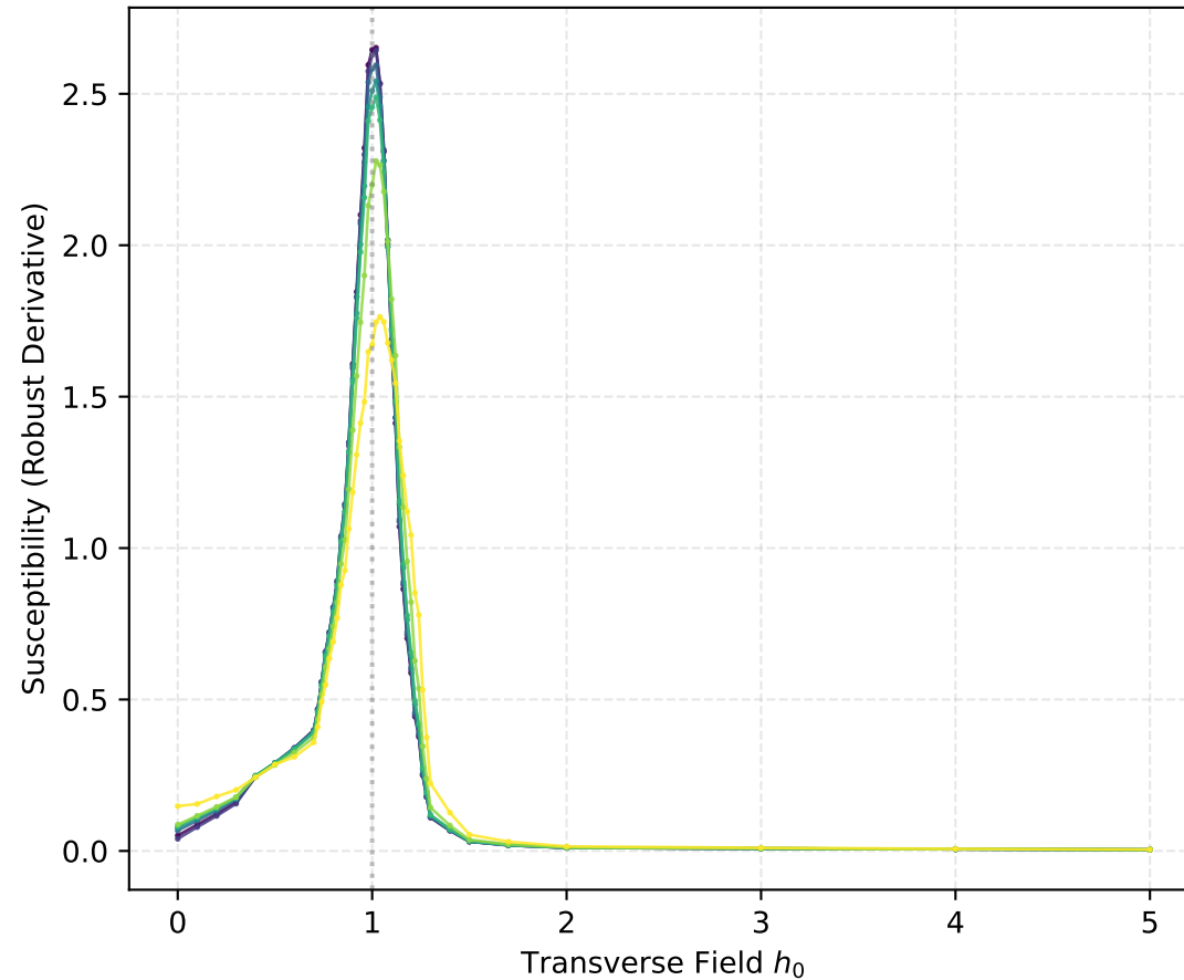
Derivative of Mean M_z^2 (span=3)
