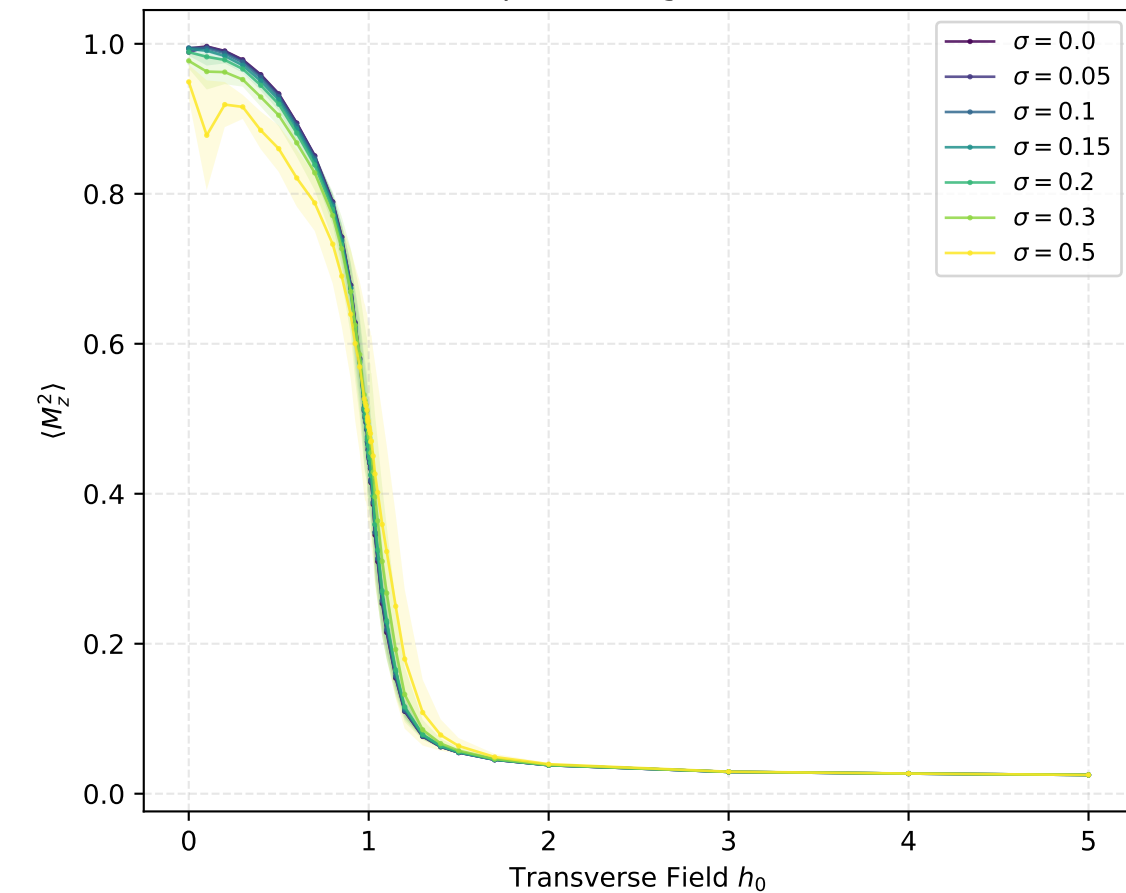
Mean Squared Magnetization (IS)
