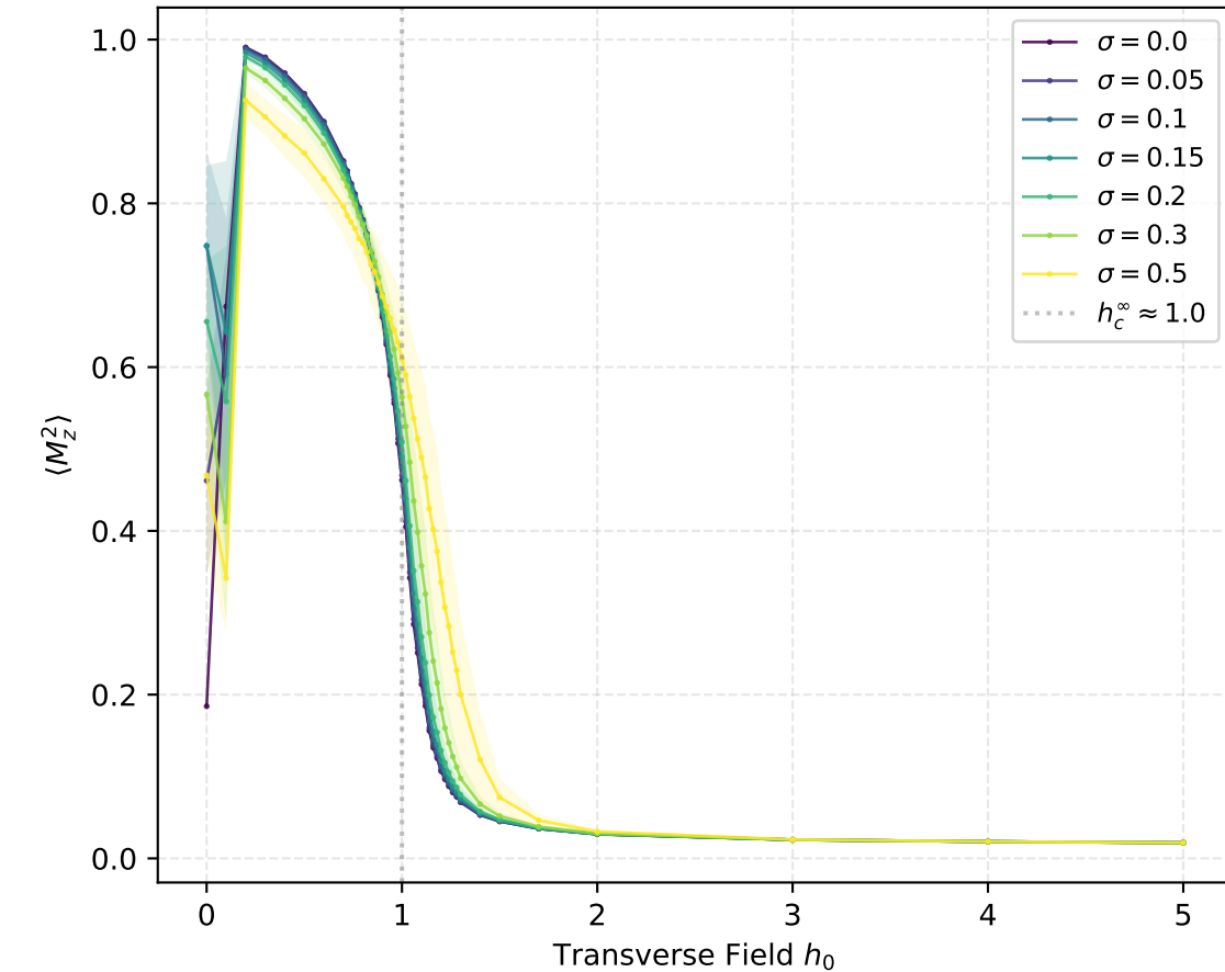
Mean Squared Magnetization — 1D L = 64 (64 spins)
