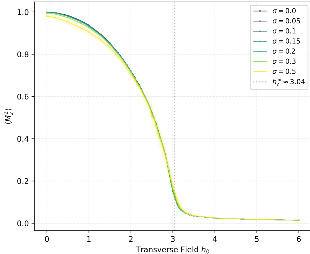
Mean Squared Magnetization — 2D L = 10 (100 spins)
