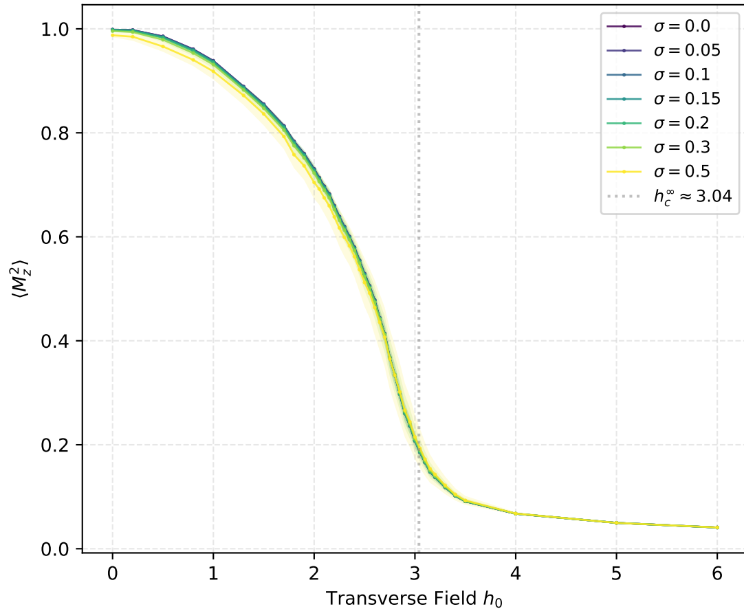
Mean Squared Magnetization — 2D L = 6 (36 spins)
