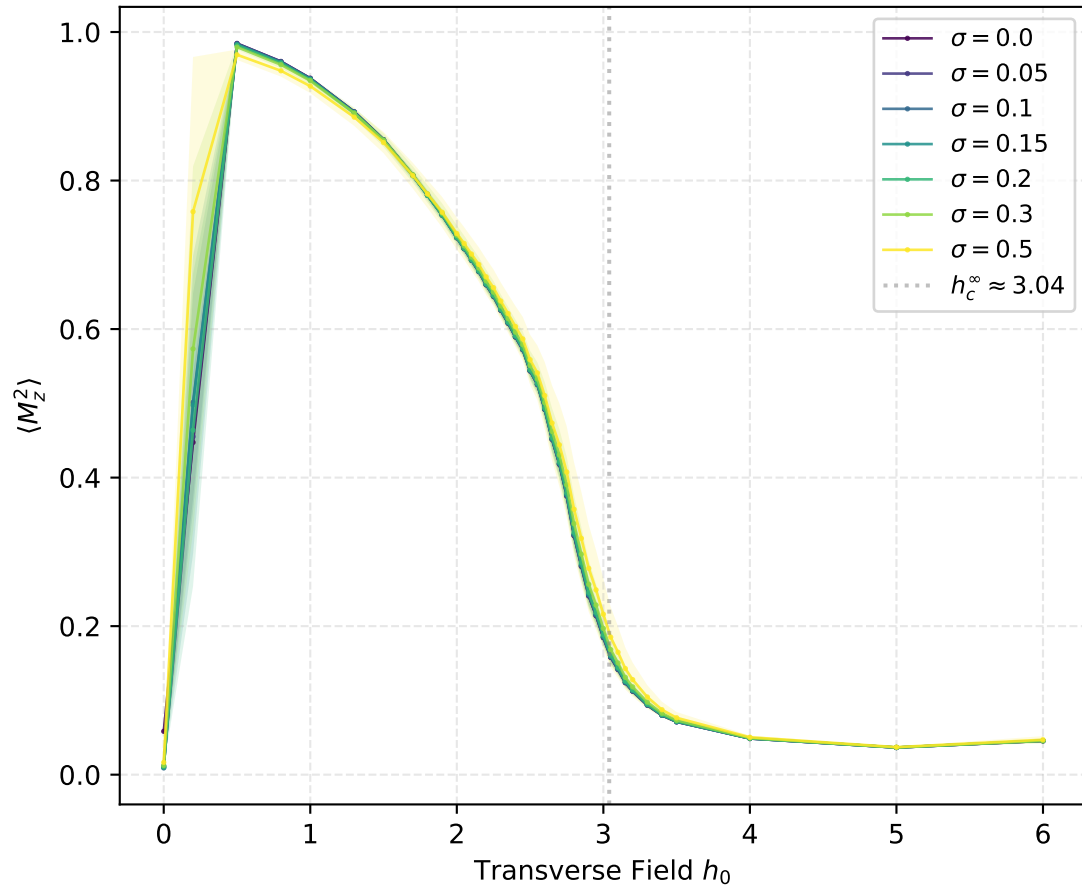
Mean Squared Magnetization — 2D L = 7 (49 spins)
