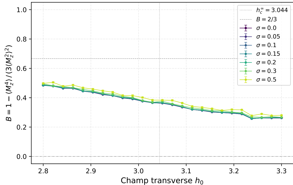
Binder cumulant — 2D TFIM, L = 5 , tous \sigma
