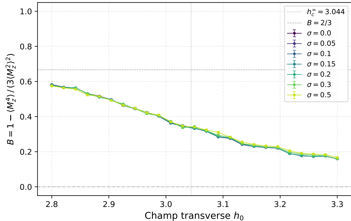
Binder cumulant — 2D TFIM, L = 8 , tous \sigma
