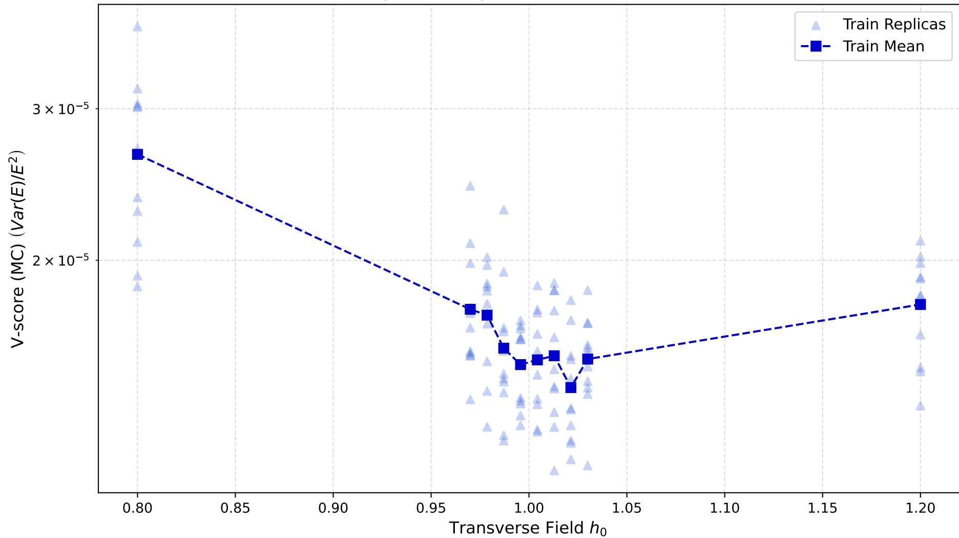
Accuracy Landscape (MC Est.): V-score (L=24)
