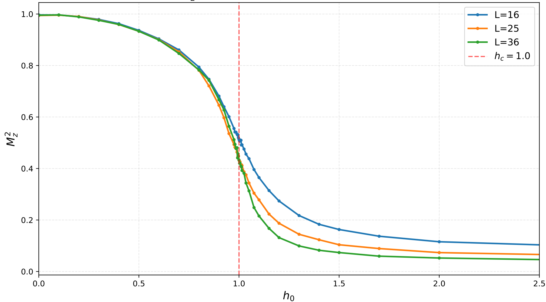
M_z^2(h) -- 1D Ising transverse, \sigma = 0
