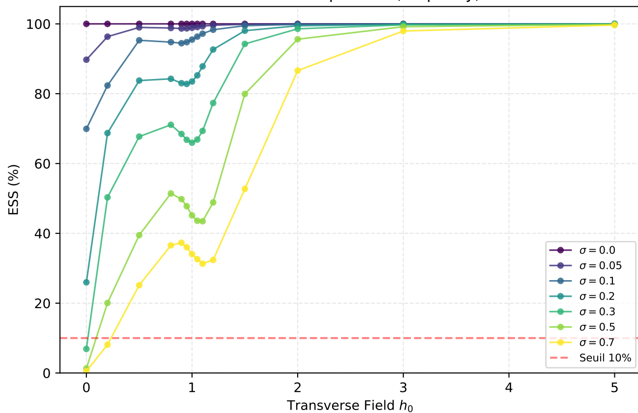
Effective Sample Size (IS quality)
