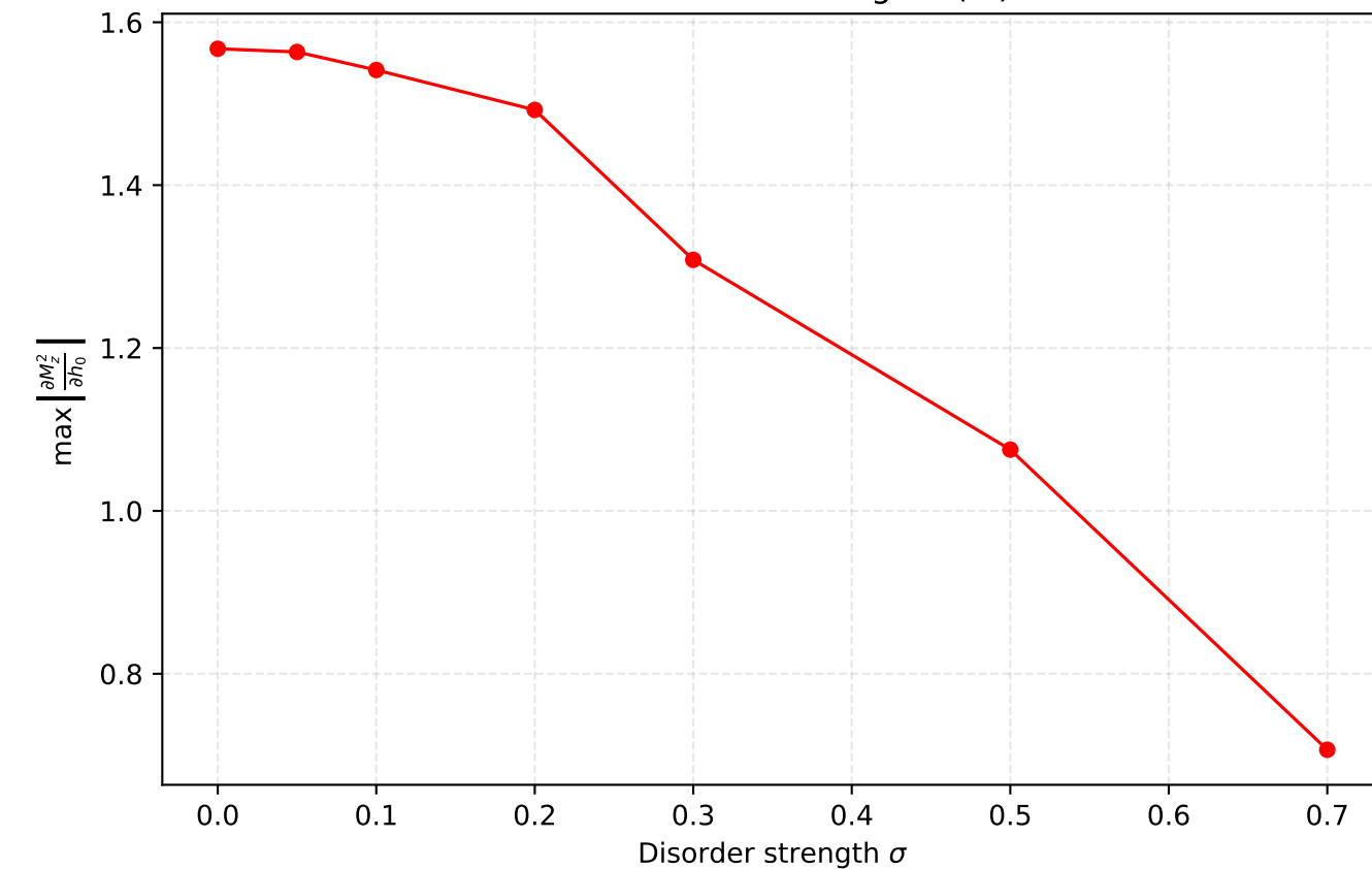
Max Derivative vs Sigma (IS)
