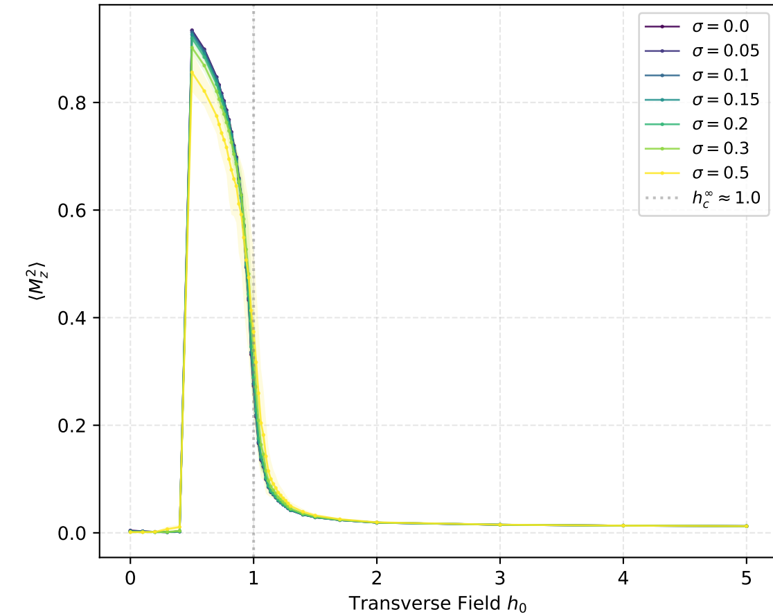
Mean Squared Magnetization — 1D L = 100 (100 spins)
