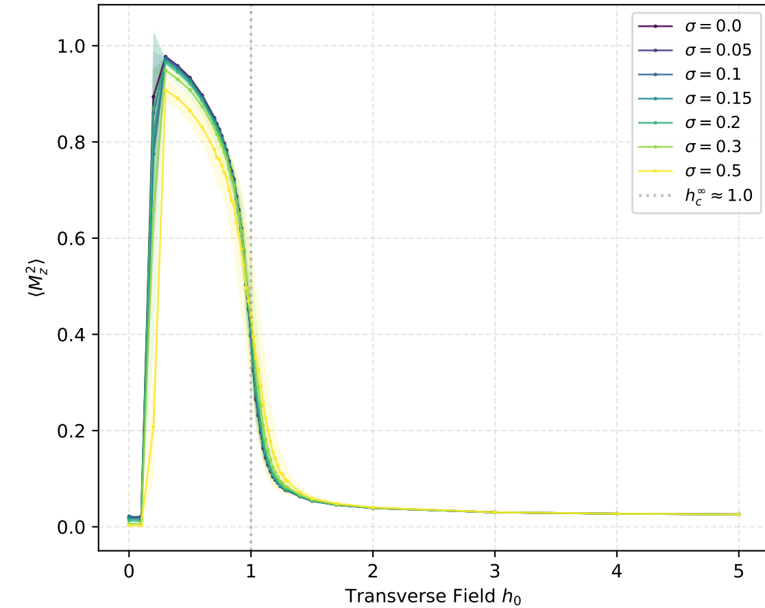
Mean Squared Magnetization — 1D L = 48 (48 spins)
