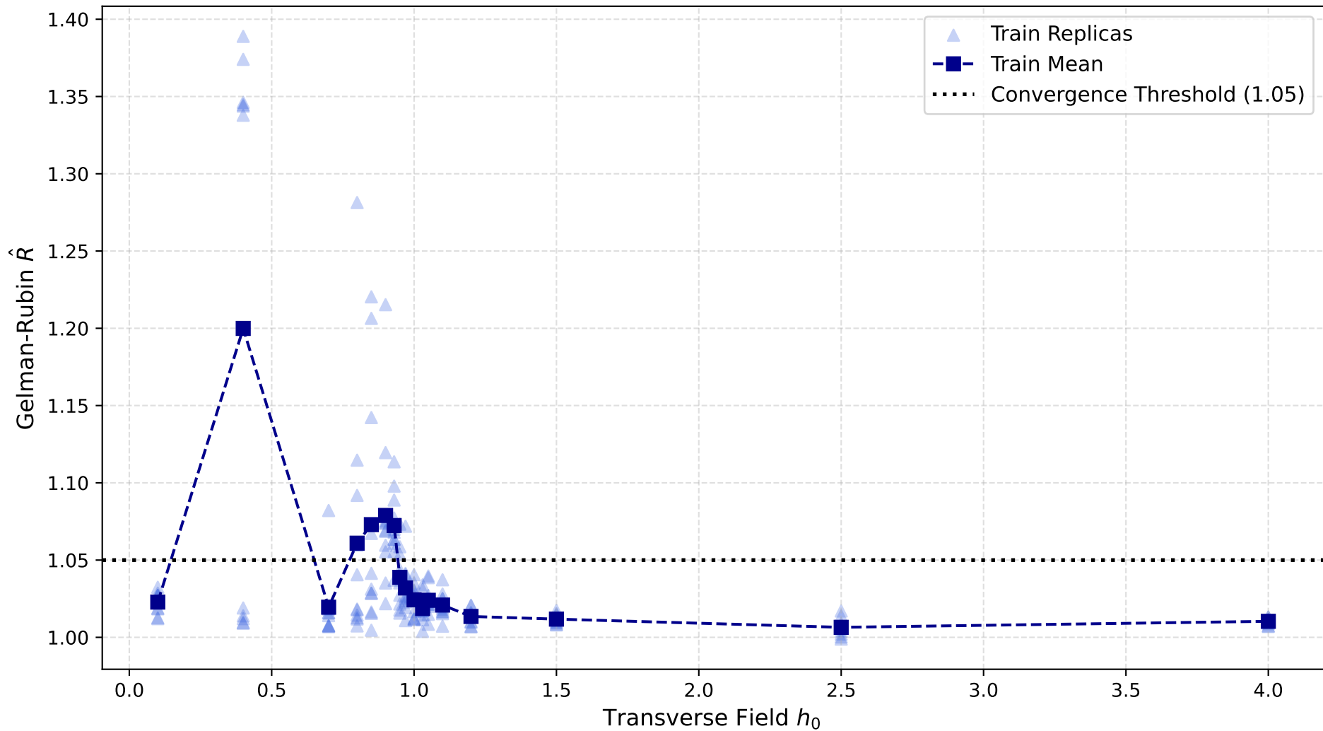
Convergence Diagnostics ( \hat{R} ): Train only (L=80)
