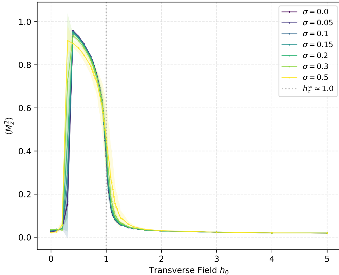
Mean Squared Magnetization — 1D L = 64 (64 spins)
