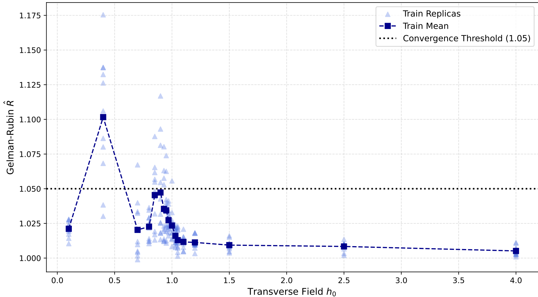
Convergence Diagnostics ( \hat{R} ): Train only (L=64)
