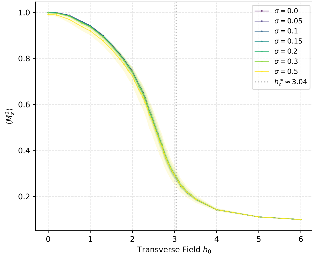
Mean Squared Magnetization — 2D L = 4 (16 spins)
