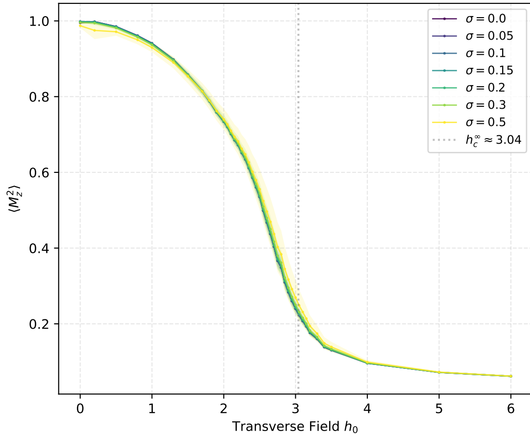
Mean Squared Magnetization — 2D L = 5 (25 spins)
