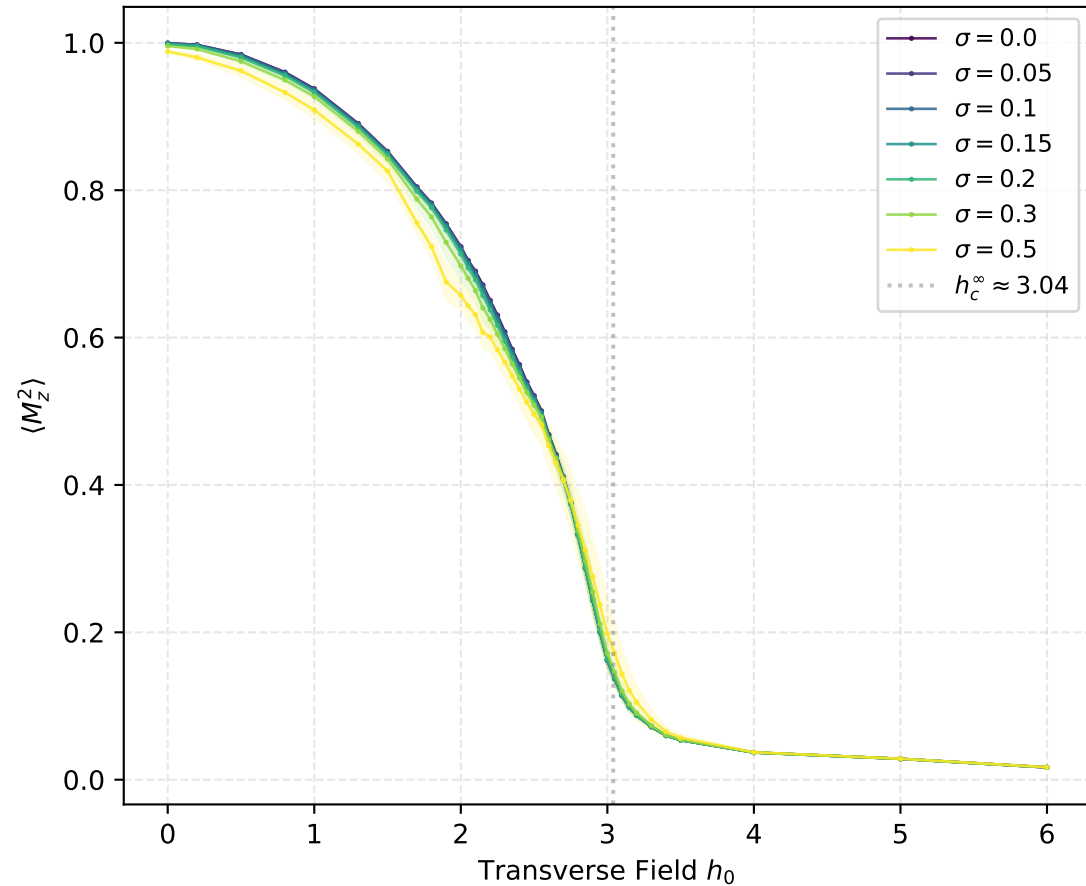
Mean Squared Magnetization — 2D L = 8 (64 spins)
