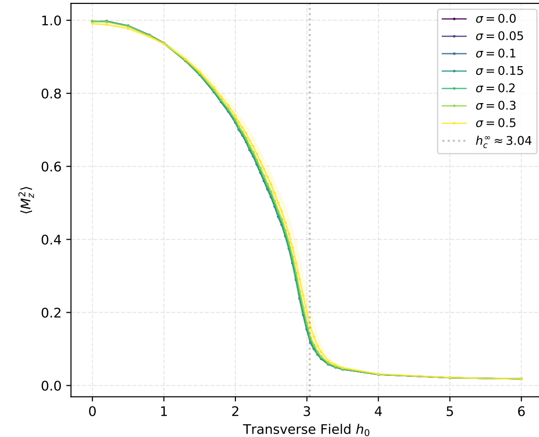
Mean Squared Magnetization — 2D L = 9 (81 spins)
