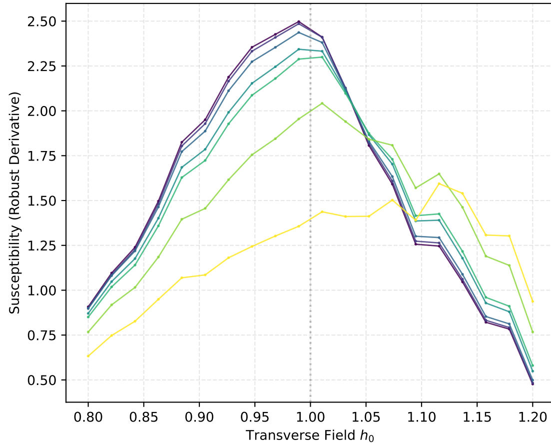
Derivative of Mean M_z^2 (span=2)
