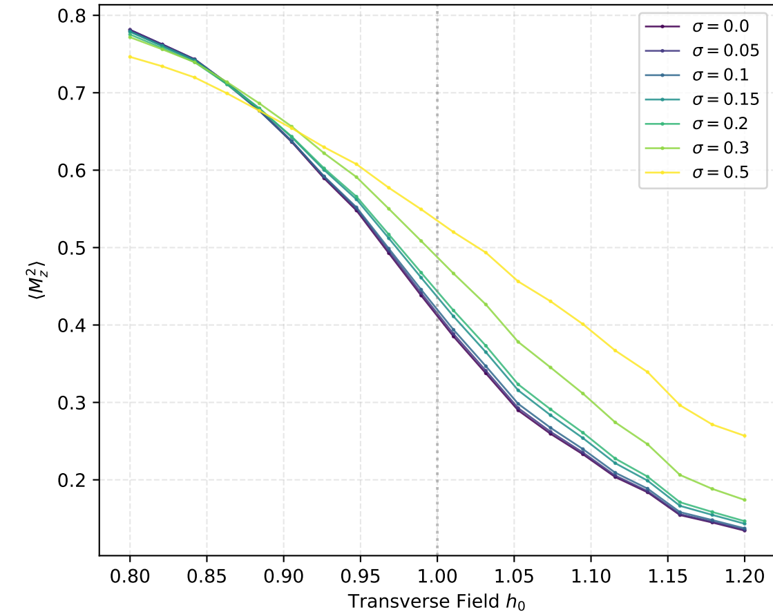
Mean Squared Magnetization — 1D L = 36 (36 spins)
