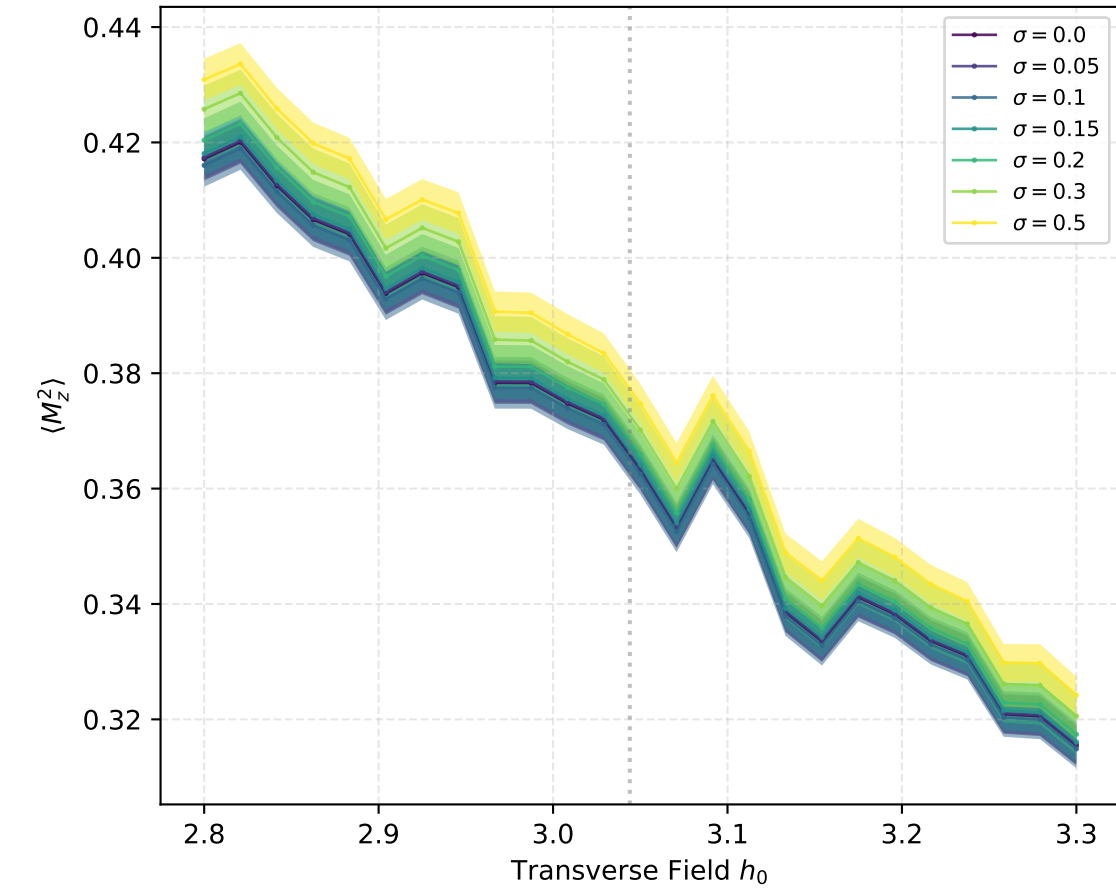
Mean Squared Magnetization — 2D L = 3 (9 spins)
