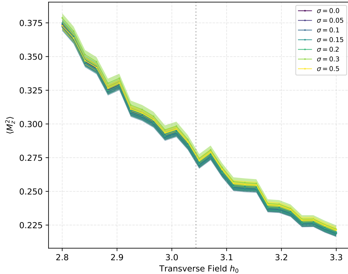
Mean Squared Magnetization — 2D L = 4 (16 spins)
