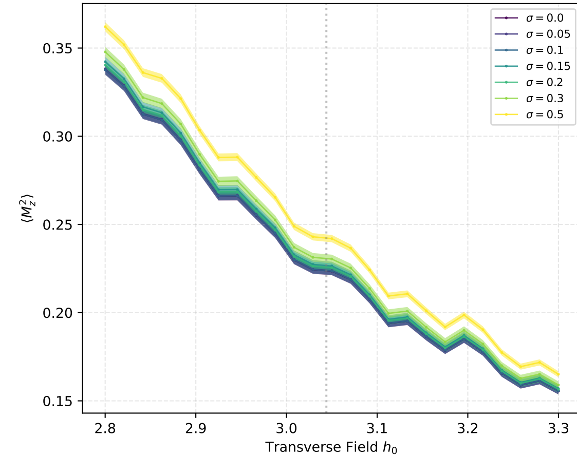
Mean Squared Magnetization — 2D L = 5 (25 spins)
