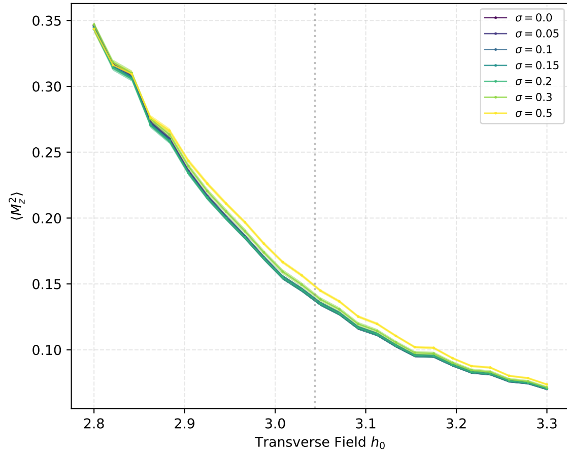
Mean Squared Magnetization — 2D L = 8 (64 spins)
