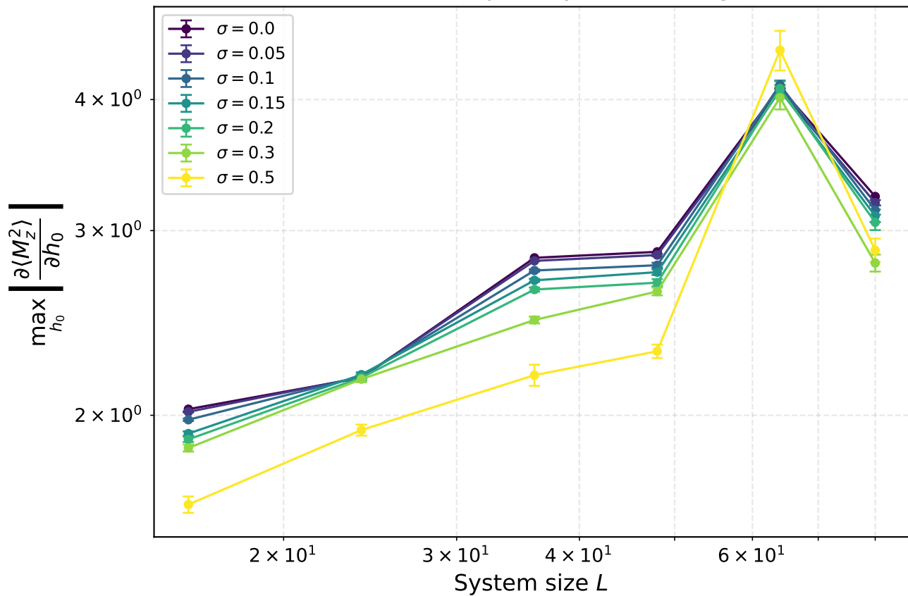
Maximum susceptibility vs L — Ising 1D
