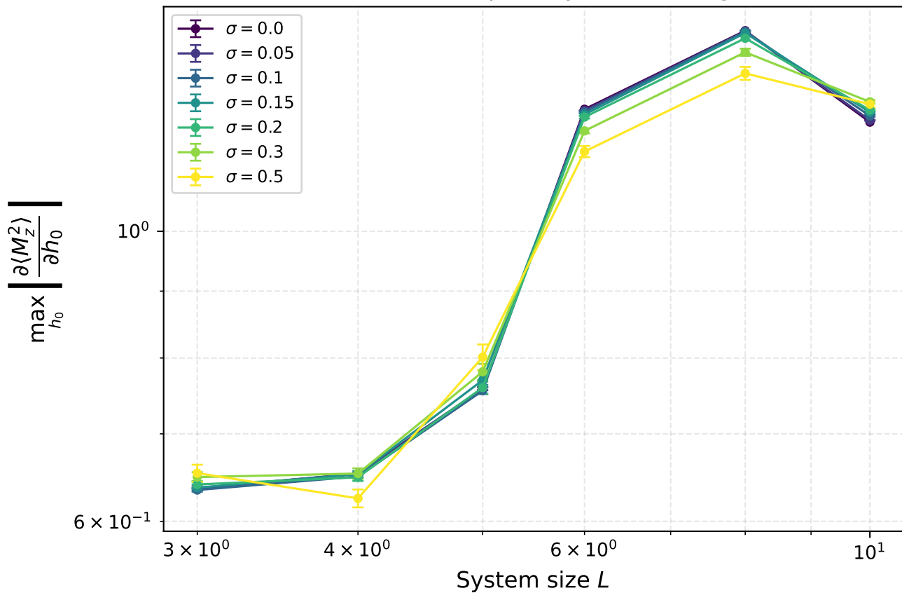
Maximum susceptibility vs L — Ising 2D
