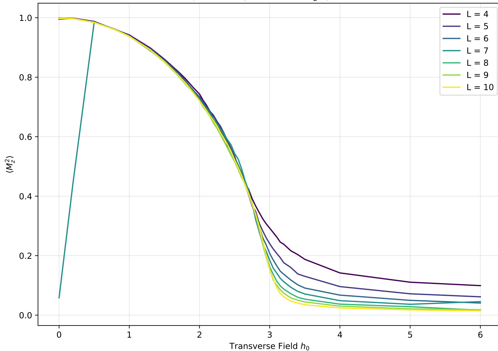
Mean Squared Magnetization \langle M_z^2 \rangle pour \sigma = 0.0
