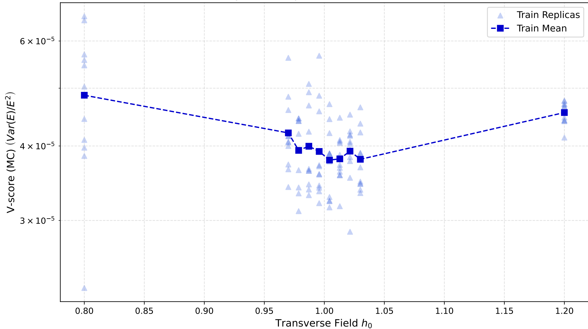
Accuracy Landscape (MC Est.): V-score (L=36)
