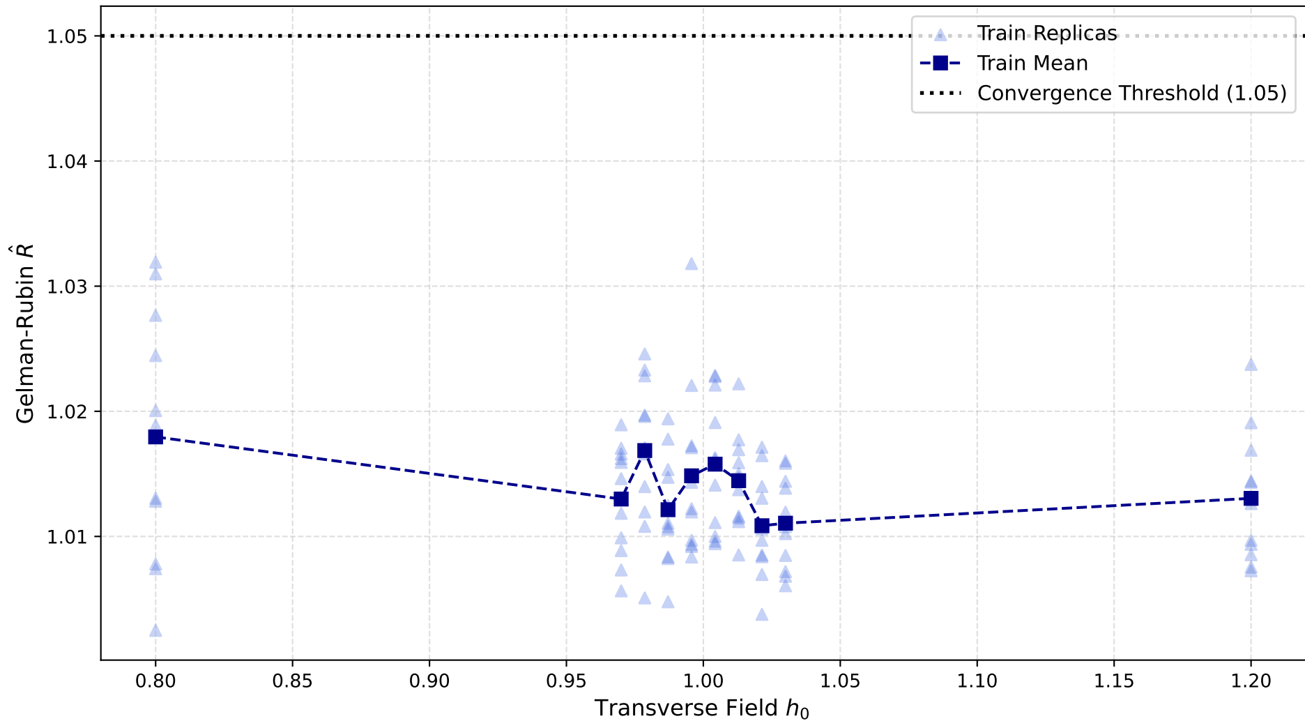
Convergence Diagnostics ( \hat{R} ): Train only (L=24)
