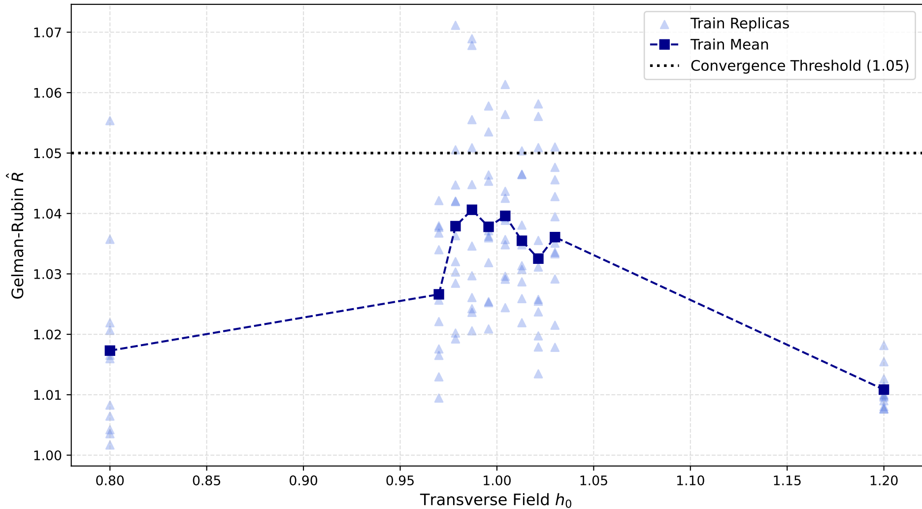
Convergence Diagnostics ( \hat{R} ): Train only (L=16)
