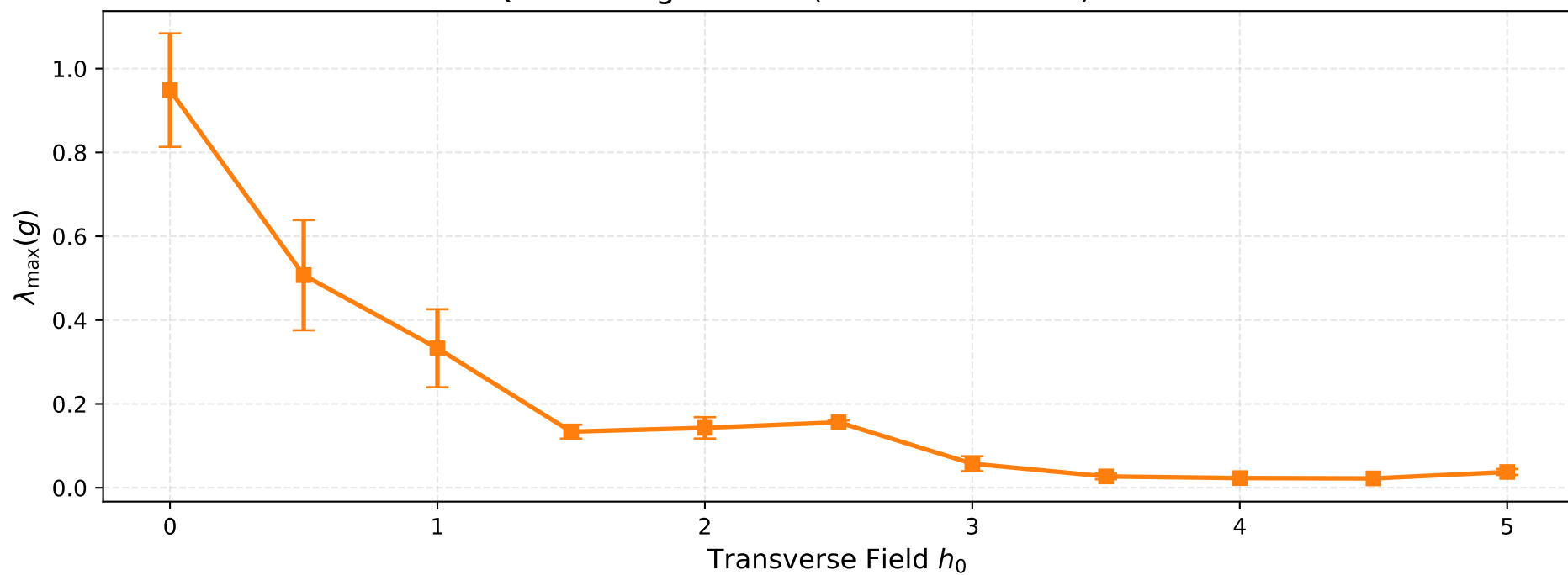
QFI Max Eigenvalue (Critical direction) - L=6
