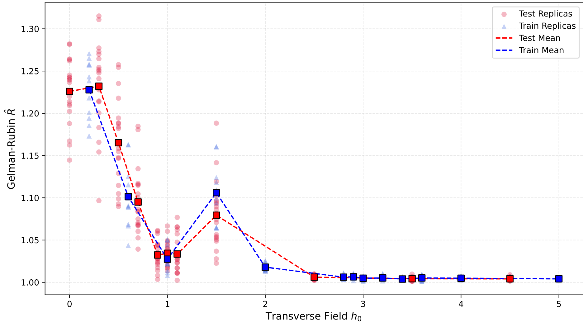
Convergence Diagnostics ( \hat{R} ): Train vs Test (Grid=6x6)
