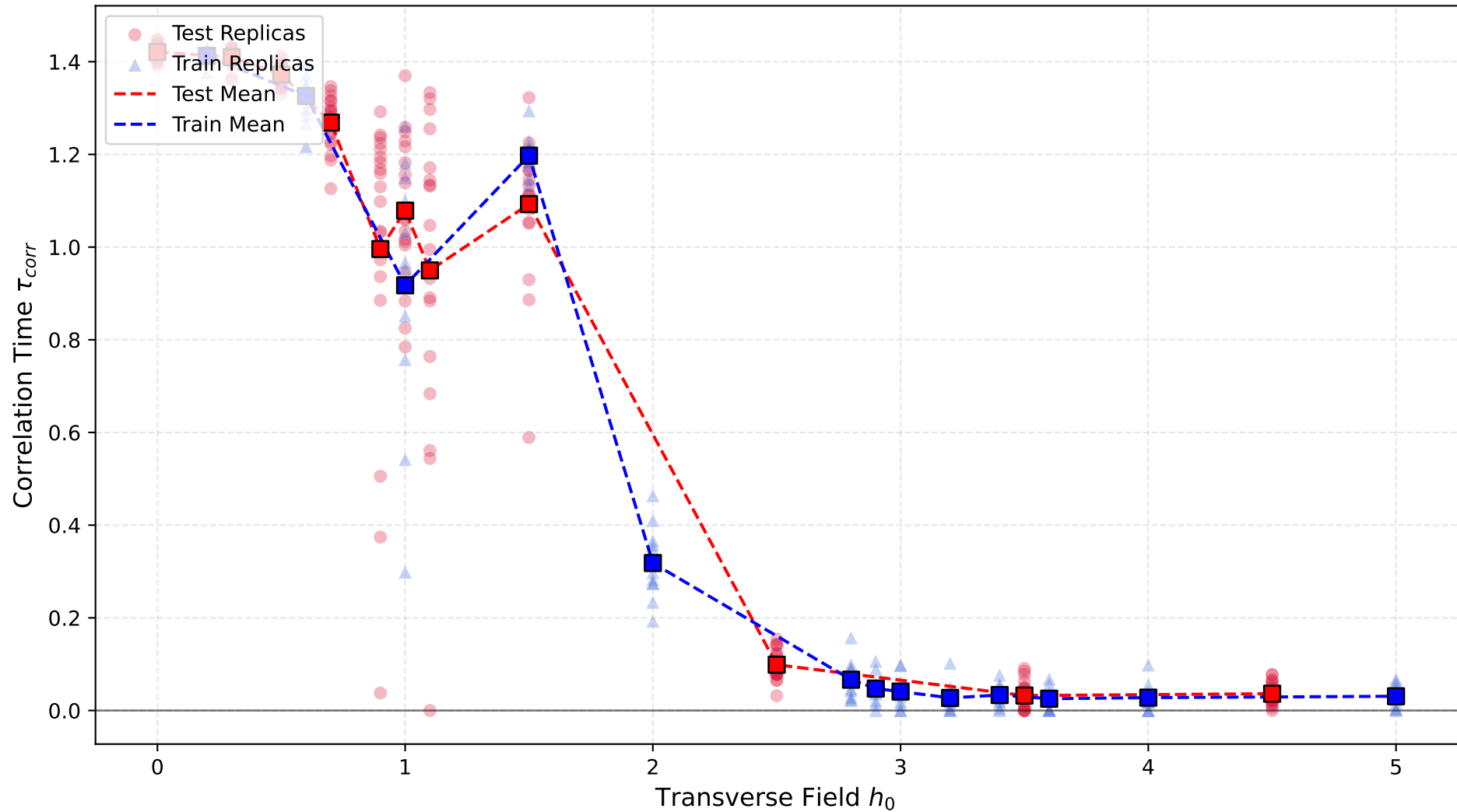
Sampling Efficiency ( \tau_{corr} ): Train vs Test (Grid=6x6)
