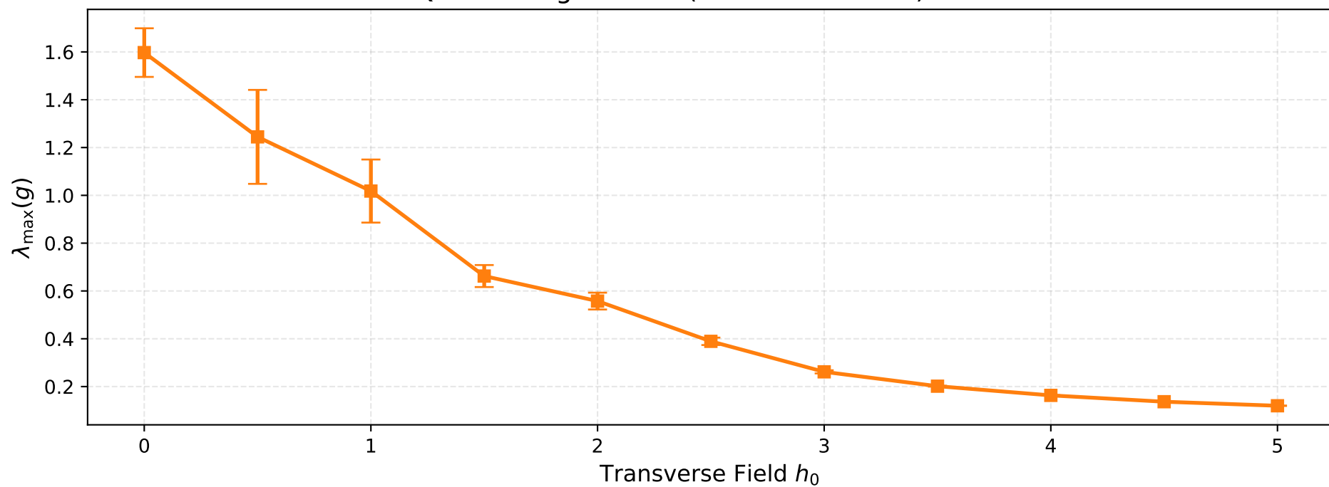
QFI Max Eigenvalue (Critical direction) - L=8
