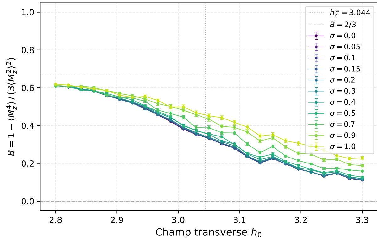
Binder cumulant — 2D TFIM, L = 10 , tous \sigma
