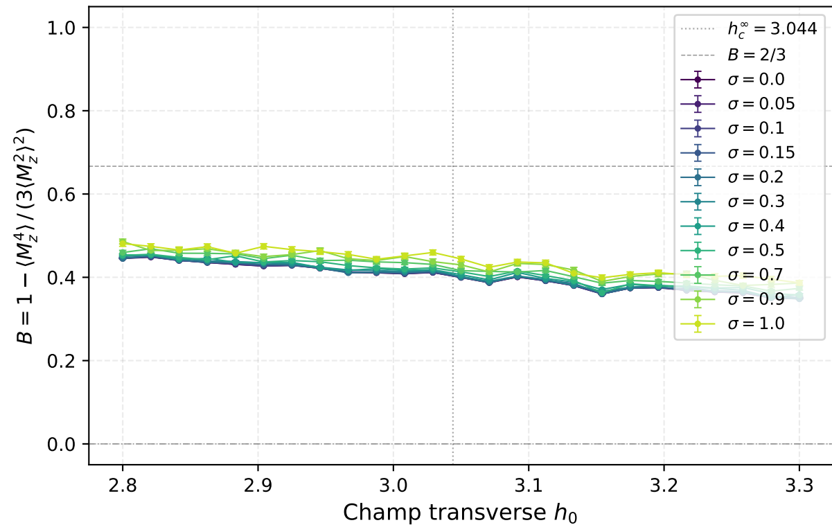
Binder cumulant — 2D TFIM, L = 3 , tous \sigma
