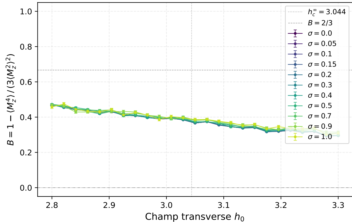
Binder cumulant — 2D TFIM, L = 4 , tous \sigma
