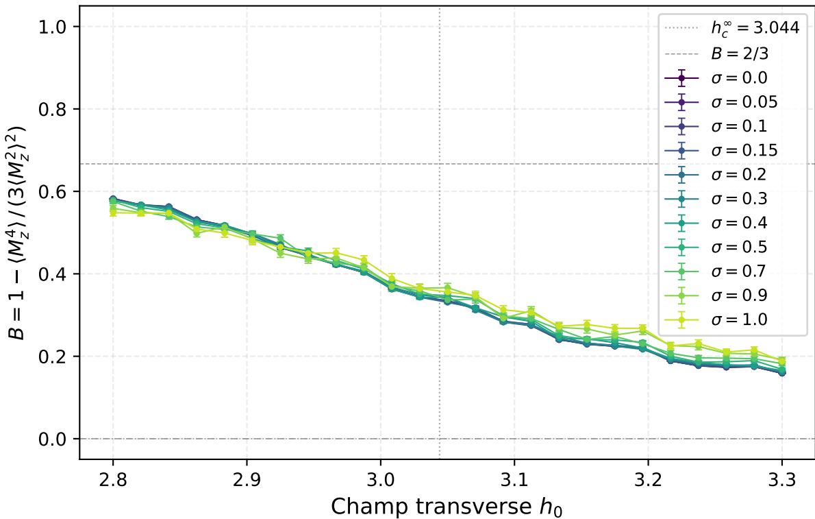
Binder cumulant — 2D TFIM, L = 8 , tous \sigma
