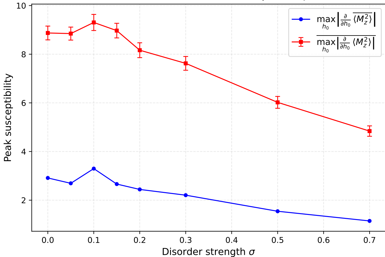
Max-of-mean vs Mean-of-max — 1D L = 25 , span=1, h_0 \in [0.5, 1.5]
